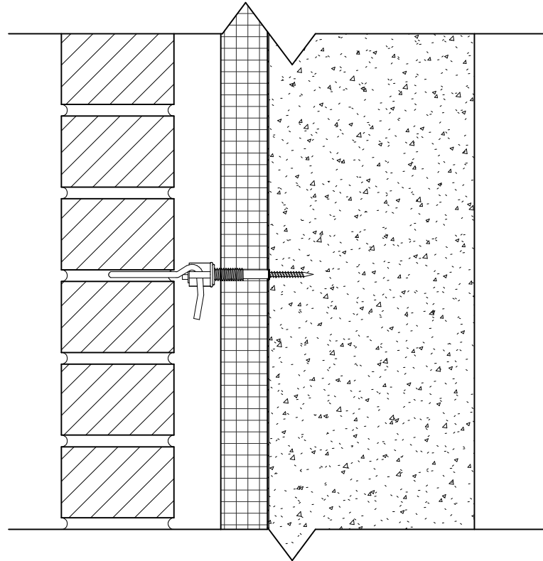
① HB-2-SEAL-WINGNUT-CONCRETE-SECTION 3" = 1'-0"
