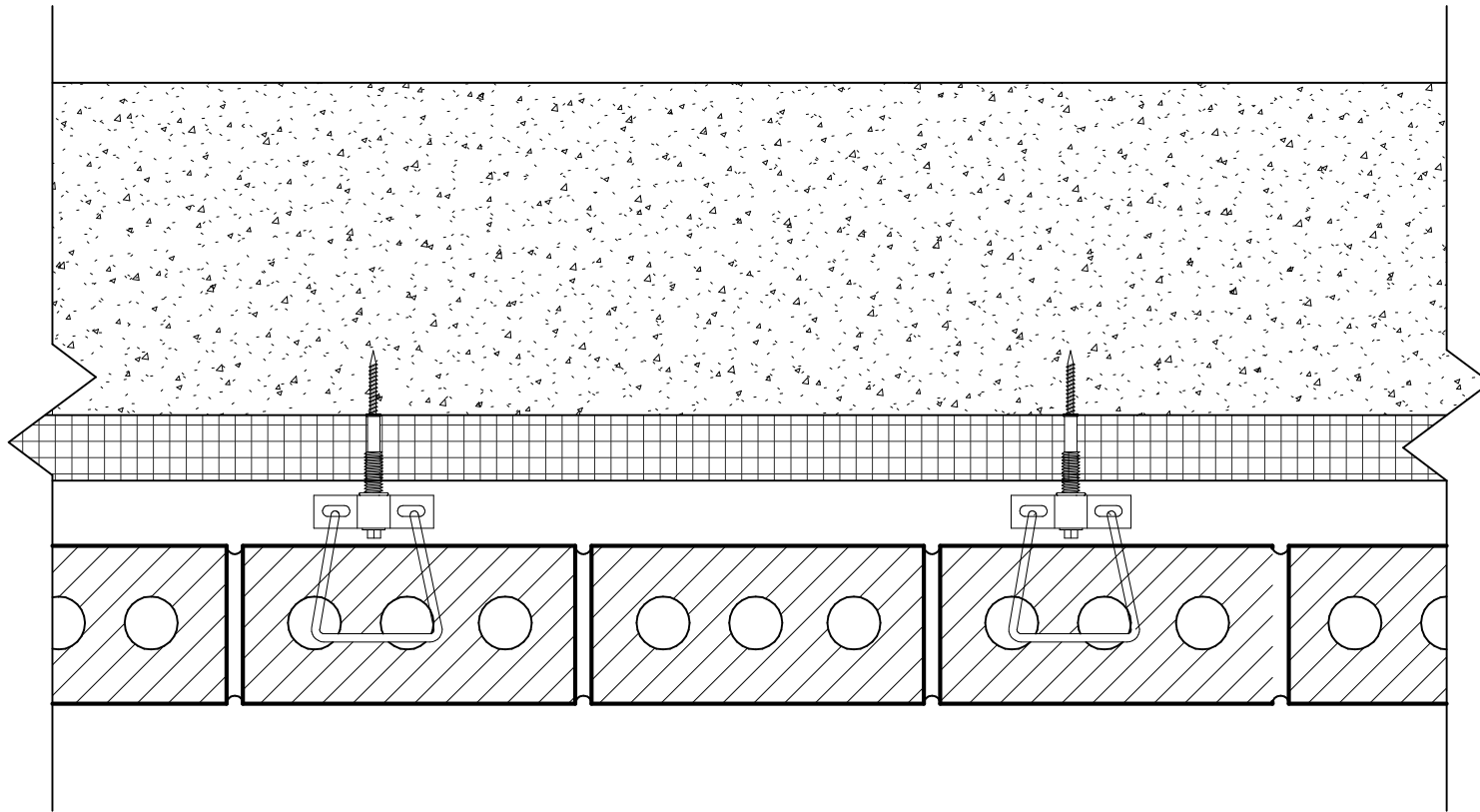
① HB-2-SEAL-WINGNUT-CONCRETE-PLAN 3" = 1'-0"
